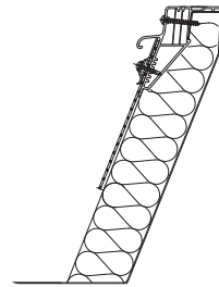
Metal upstand ISO-THERM Model, 30 cm high with E-clamping rail
